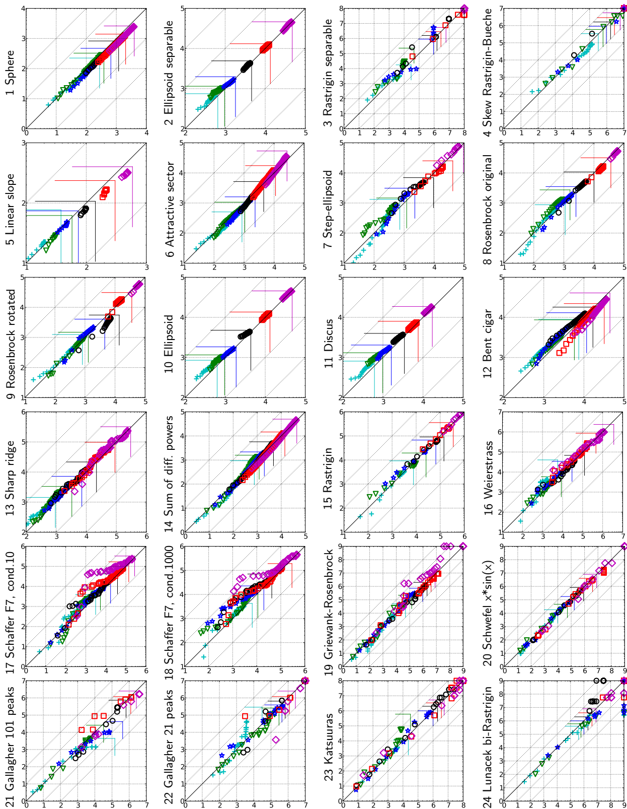
Figure 2: Expected running time (ERT in \log_{10} of number of function evaluations) of CMA ma ( x -axis) versus CMA mah ( y -axis) for 46 target values \Delta f \in [10^{-8}, 10] in each dimension on functions f_1 – f_{24} . Markers on the upper or right edge indicate that the target value was never reached. Markers represent dimension: 2: +, 3: ▽, 5: *, 10: ○, 20: □, 40: ◇.
